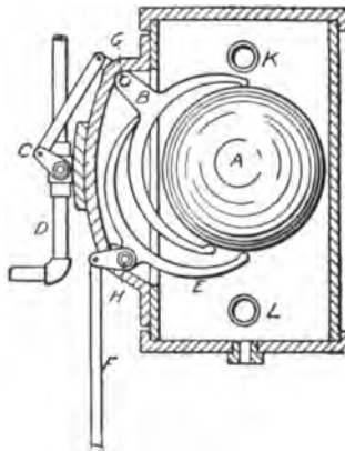
FIG. 191.—The Keene Automatic Water Level Regulator. The ball, A, floating in the water at boiler level; B and E contact fingers, or pivots; G and H, operating the valve, C, on water pipe, D, and the fuel valve through the link, F.
